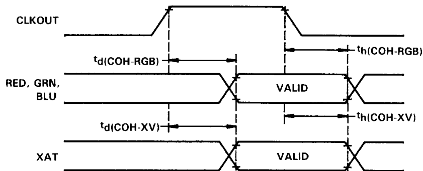
(a) PHASE A VIDEO OUTPUTS
