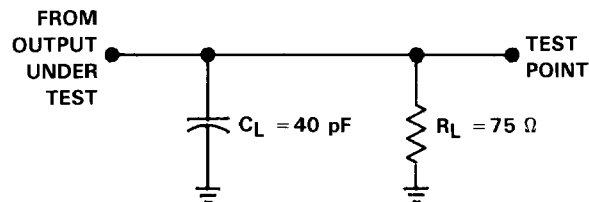
FIGURE 3. TEST LOAD CIRCUIT—ANALOG OUTPUTS
