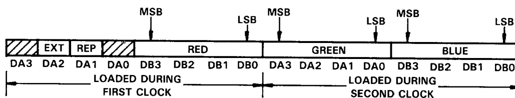
FIGURE 1. COLOR LOOKUP TABLE REGISTER
