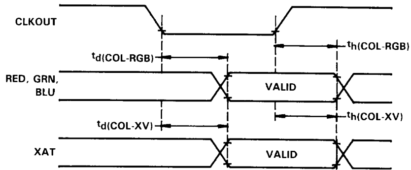
(b) PHASE B VIDEO OUTPUTS
