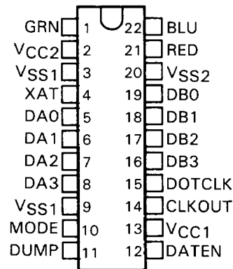
N PACKAGE (TOP VIEW)
