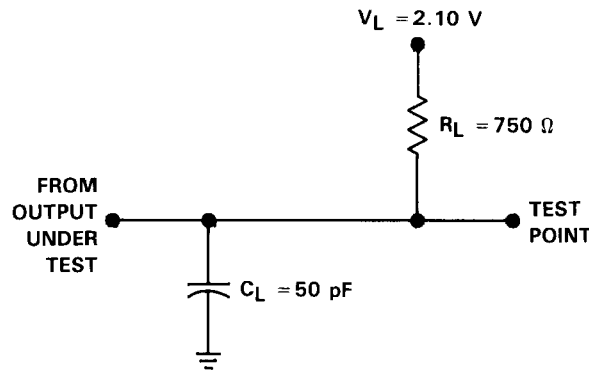
FIGURE 2. TEST LOAD CIRCUIT—DIGITAL OUTPUTS
